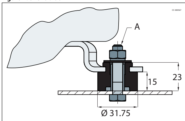
Figure 8: Terminal box
