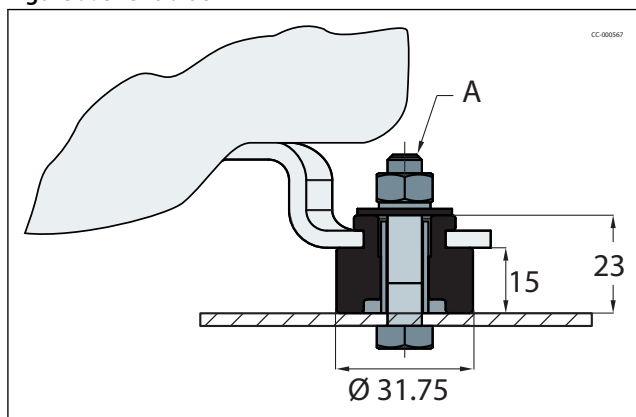
Figure 10: Terminal box for model (1)
