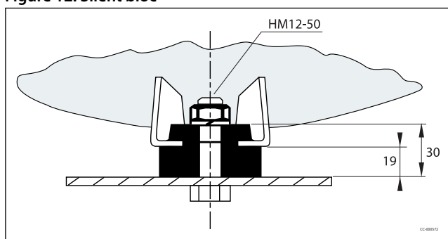
Figure 12: Silent bloc
